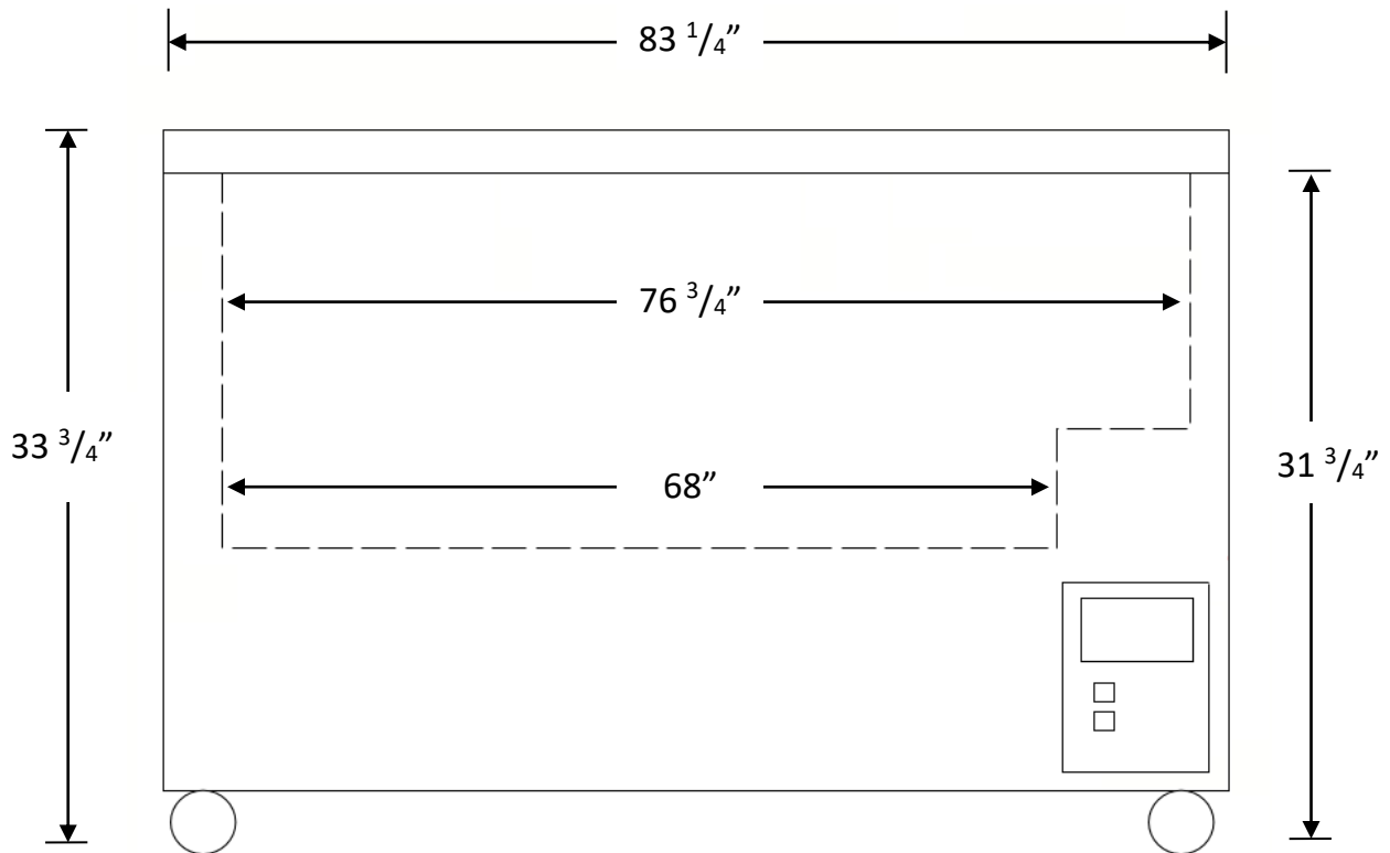
Chest Freezer Front View
